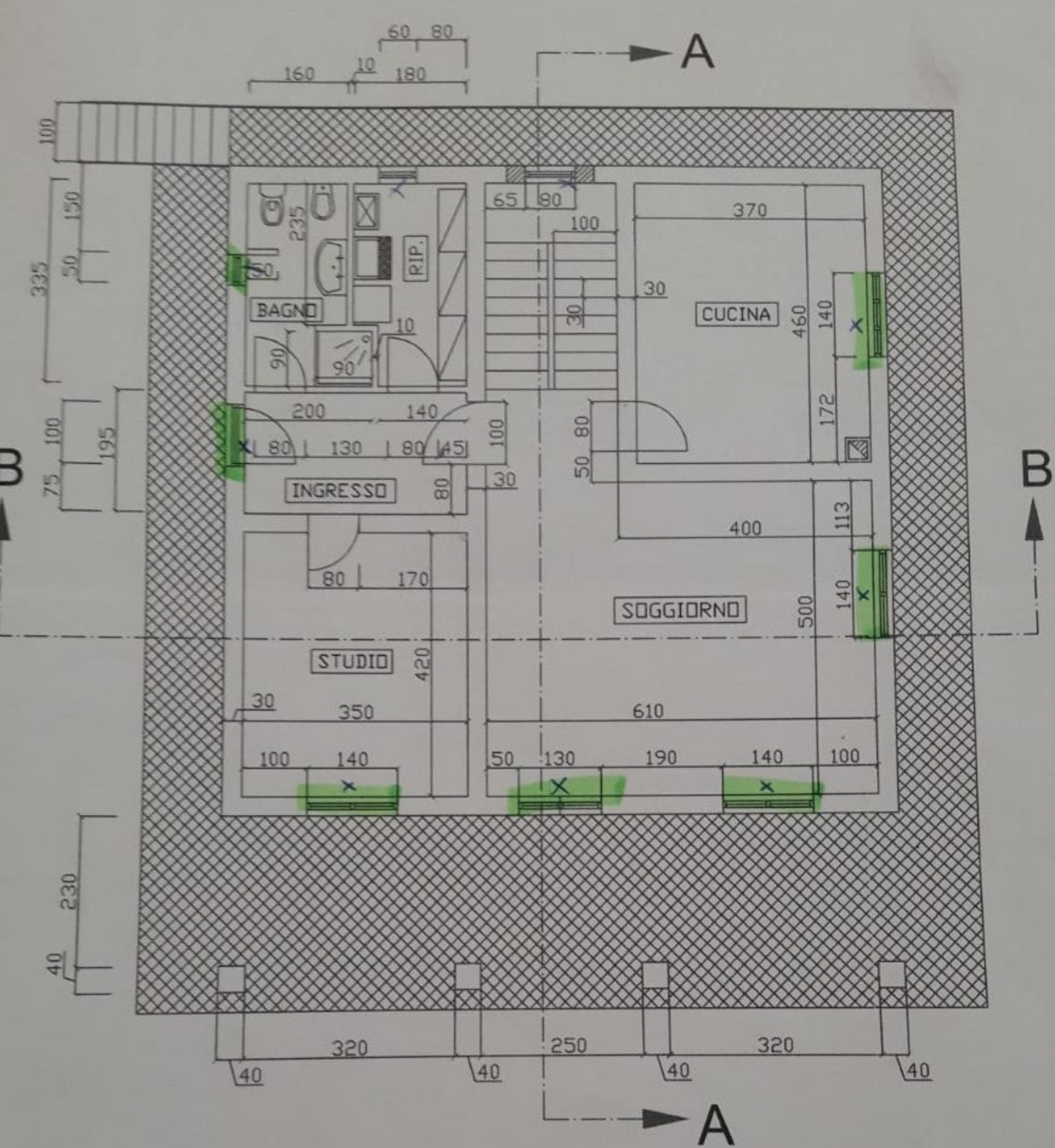
PIANO TERRA
