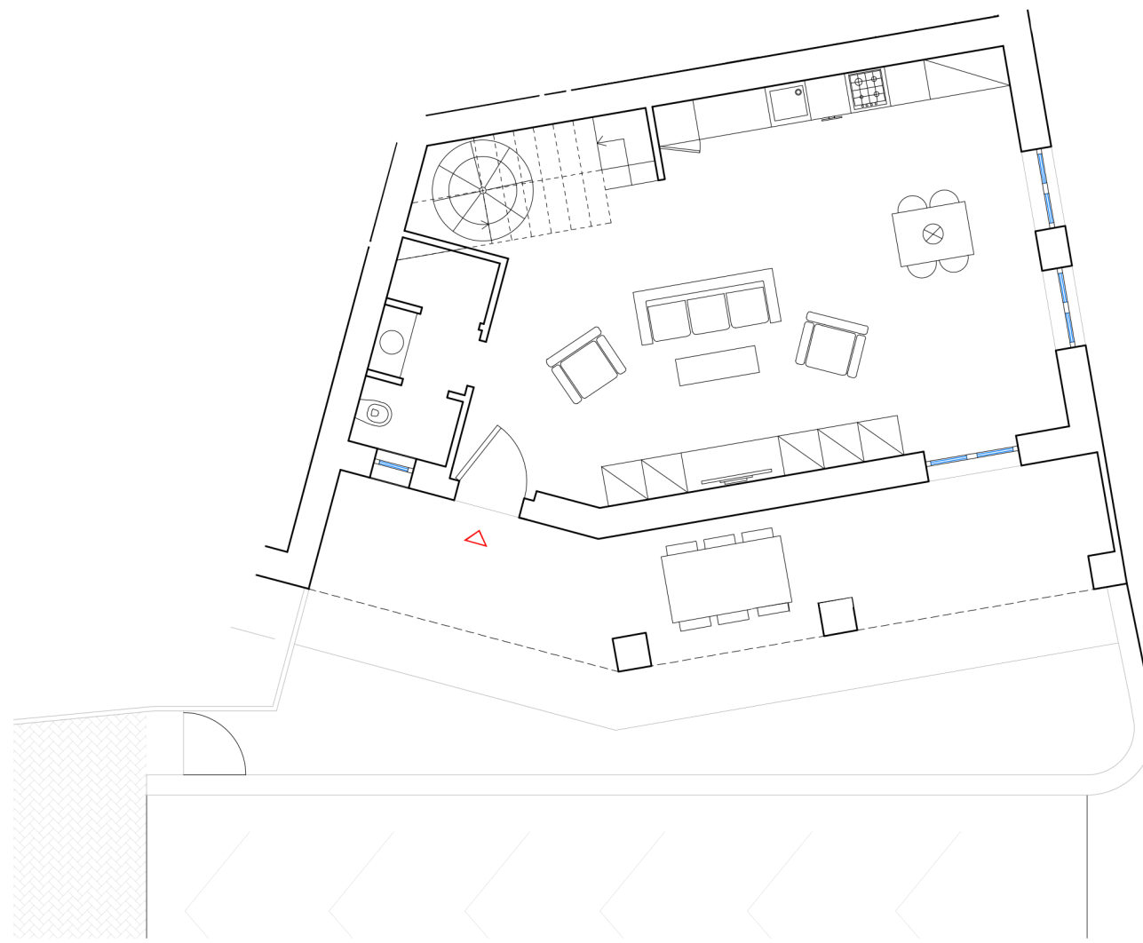
PIANO TERRA
